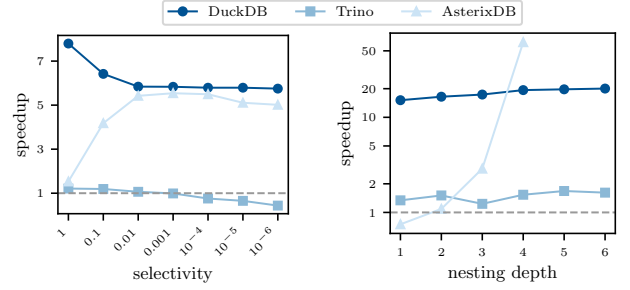
Figure 15: Speedup of manually joined approach with growing selectivity.
