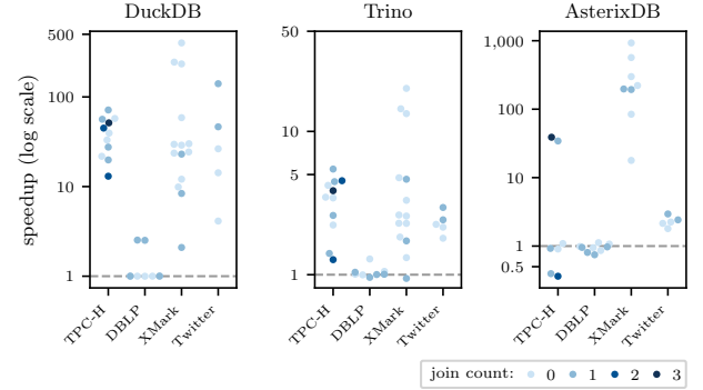
Figure 13: Speedup of manually joined normalized datasets over built-in versions of DuckDB, Trino, and AsterixDB. The colors depict the number of generated joins in the query.
