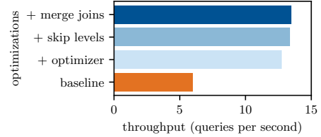
Figure 10: Performance improvements of optimizations on the entire benchmark set from Table 1. Query optimizer, skip levels, merge joins instead of hash joins.
